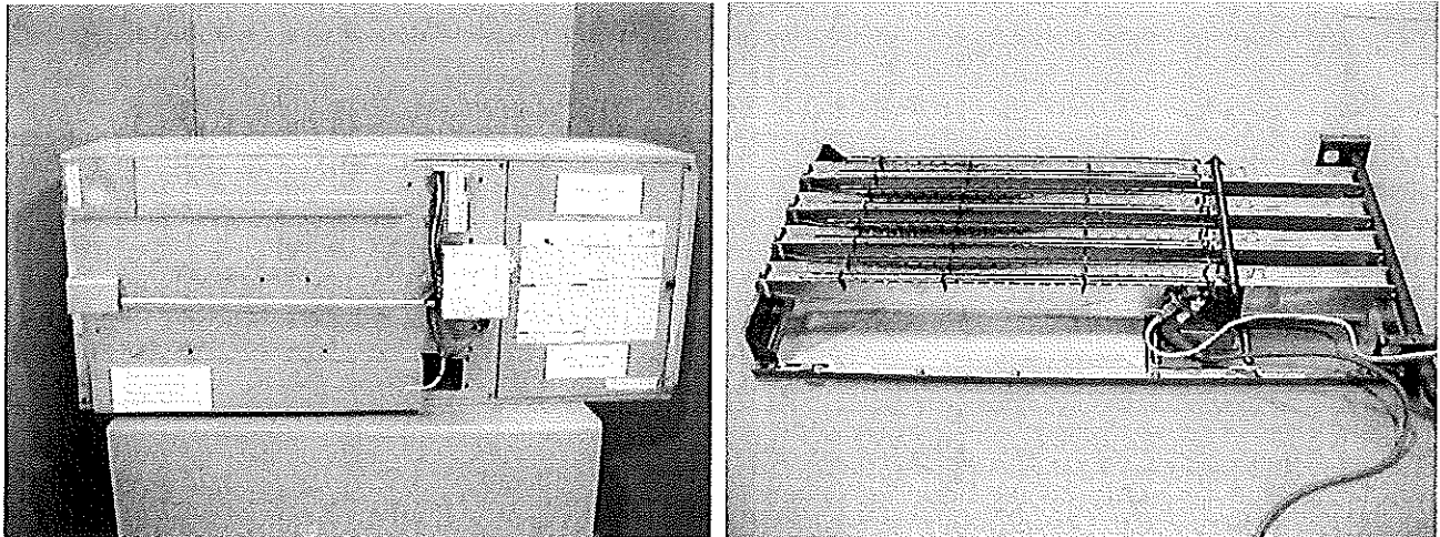
These gas-fired horizontal furnaces have steel rods (right) installed above the burners.
